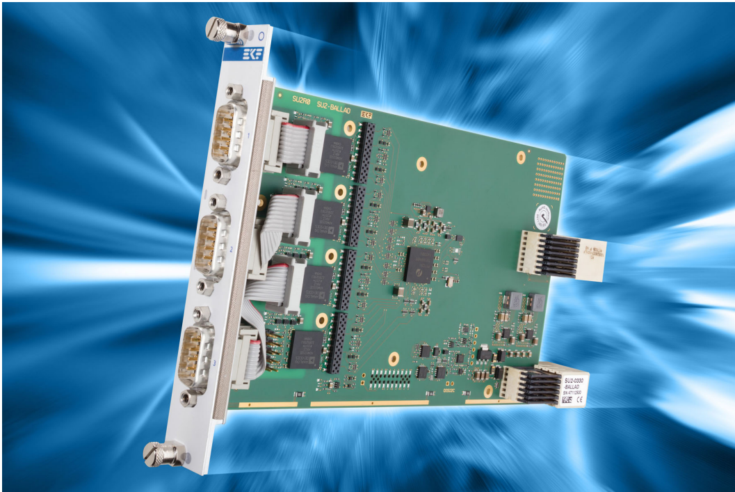
SU2-BALLAD w. Triple Standard D-Sub 4HP
