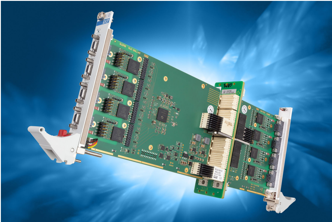
SU2-BALLAD w. SUB-RIO (8 Port 4HP Isolated RS-232)
